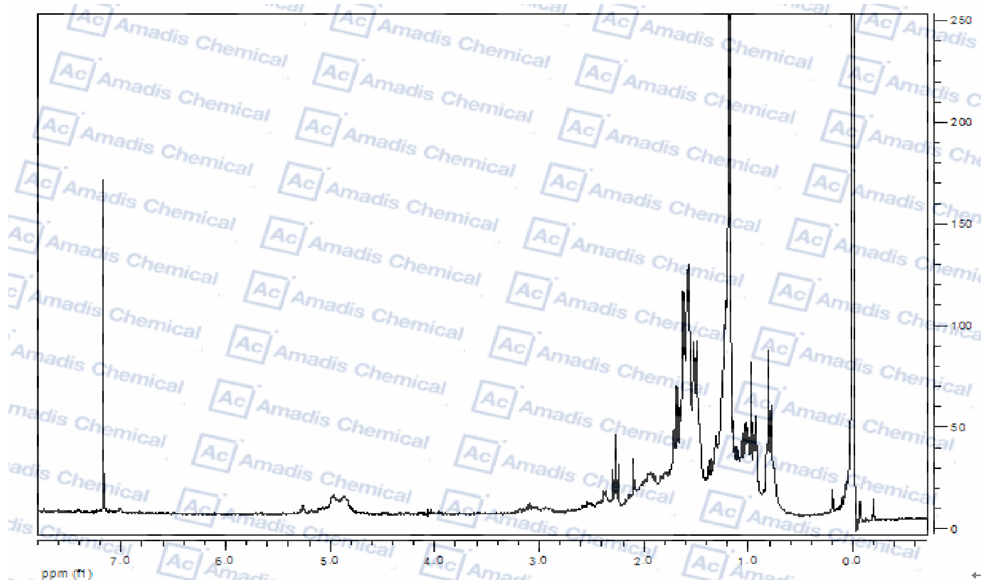
H-NMR spectrum of Hyperforin
