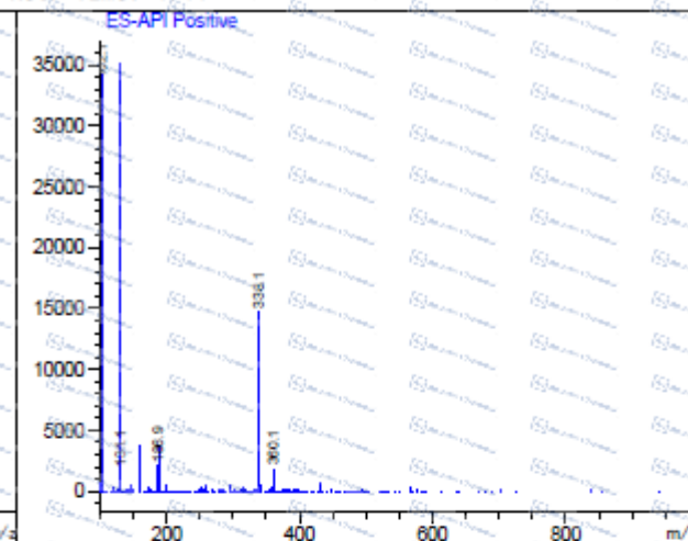
Ret. Time: 5.68
