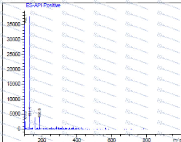
Ret. Time: 5.29
