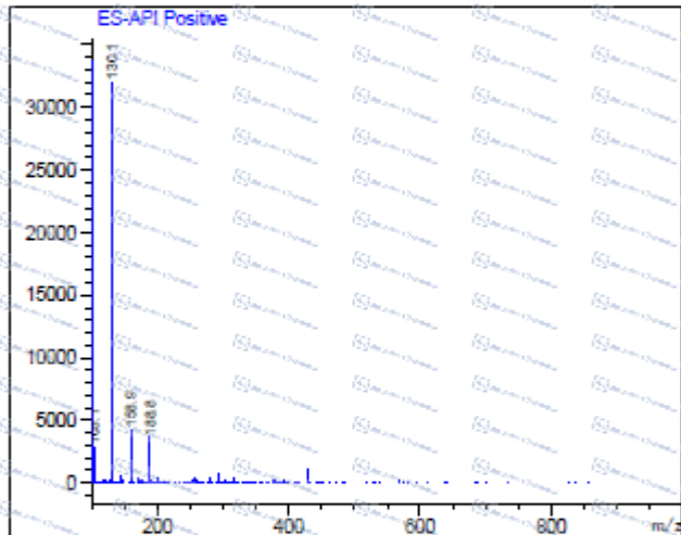
Ret. Time: 5.89
