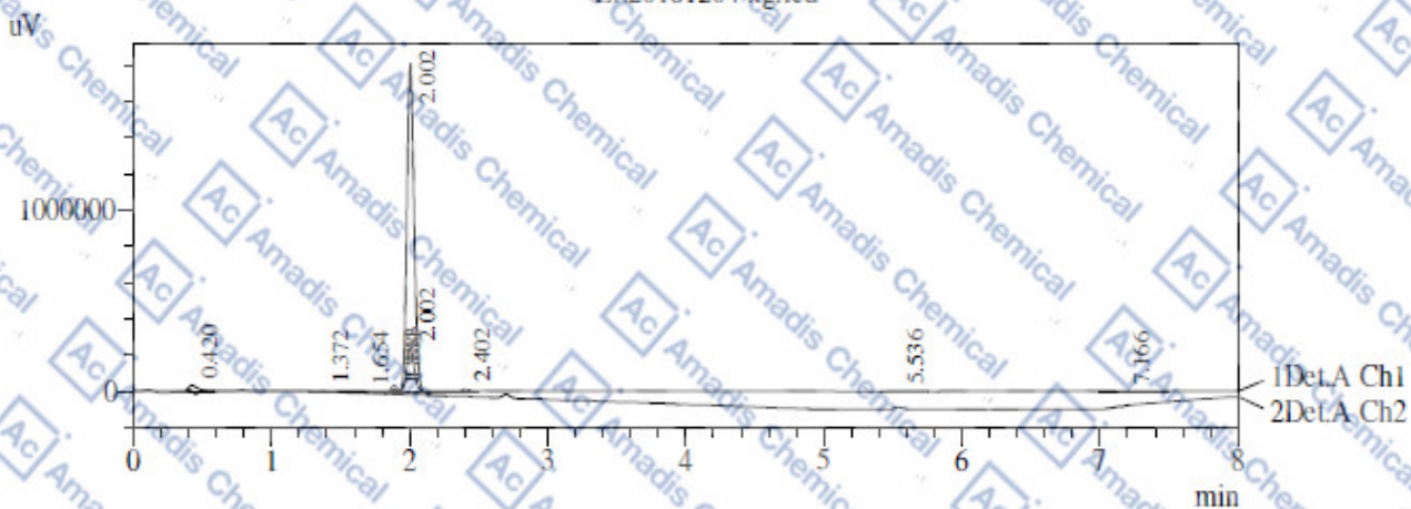
Chromatogram EA20181204-xg.lcd
